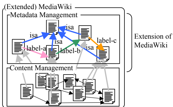
Figure 2: Semantic MediaWiki as an integrated system for content management and metadata management
