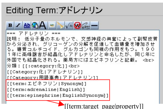
Figure 1: Editing Box of the Wiki page
