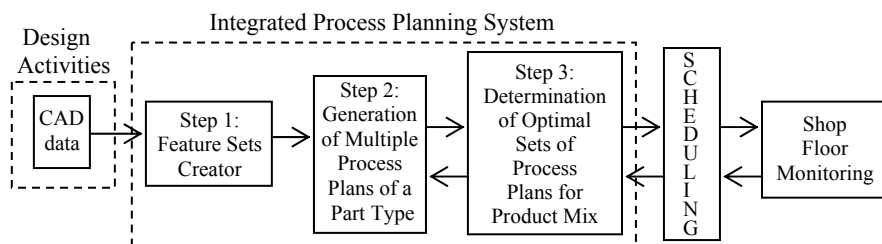
Figure 1: Overview of Integrated Computer-Aided Process Planning System
