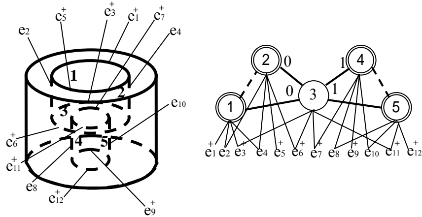
Figure 3: Stepped-hole feature and its Extended SRG representation
