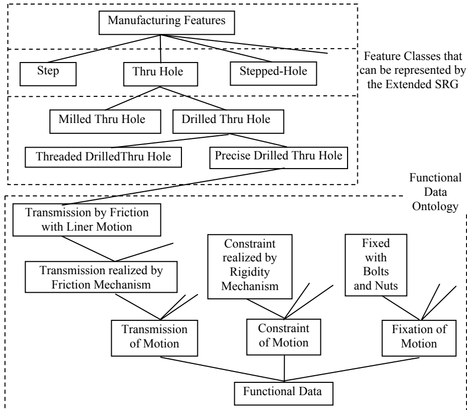
Figure 4 Ontology of manufacturing features and functional data
