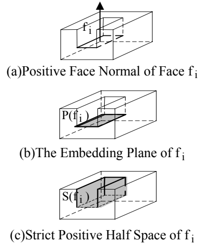
Figure 2: Explanation of terms used in Extended SRG Method
