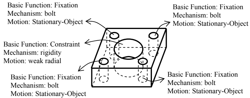
Figure 5: A sample part and the functions of the face elements
